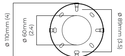
mounting plate dimensions
